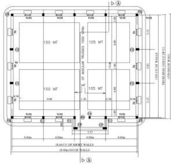
PLAN FOR (510 MT) WH. BLDG.
